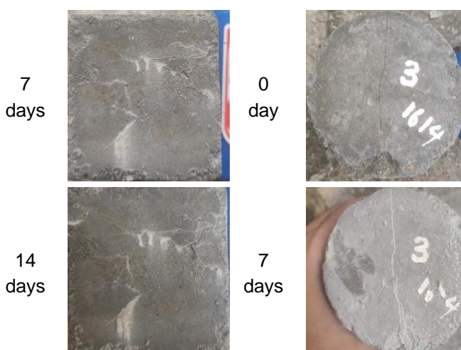
Fig 7. Healing ability of mortar mixture containing bacillus subtilis 2.57 \times 10^9 \text{ cfu/g}
