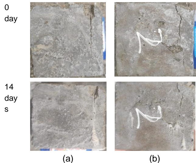
Fig 8. Healing ability of mortar mixture containing bacillus subtilis 2.05 \times 10^{10} \text{ cfu/g}
