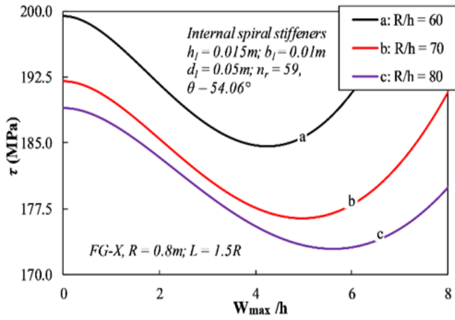
Fig 5. Comparison of dimensionless deflection – torsional load postbuckling curves spiral stiffened FG-GPLRC shells with different R/h ratios
