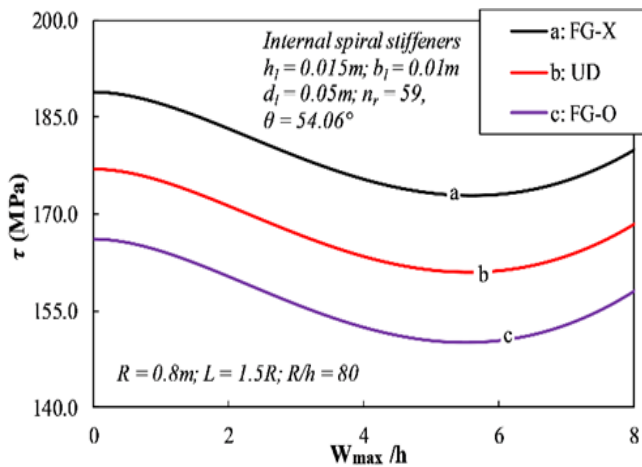
Fig 7. Comparison of dimensionless deflection – torsional load postbuckling curves of spiral stiffened FG-GPLRC cylindrical shells with different distribution laws of graphene platelet
