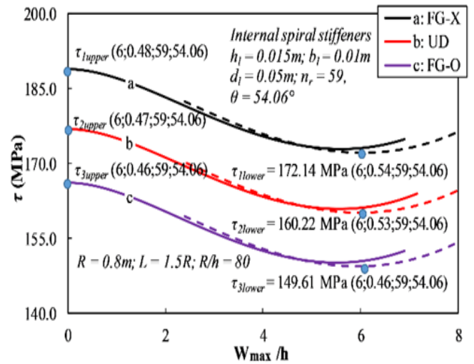
Fig 9. Upper and lower critical buckling load at the dimensionless deflection – torsional load postbuckling curves of spiral stiffened FG-GPLRC cylindrical shells
