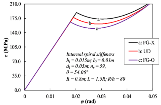
Fig 8. Comparison of torsional angle – torsional load postbuckling curves of spiral stiffened FG-GPLRC cylindrical shells with different distribution laws of graphene platelet
