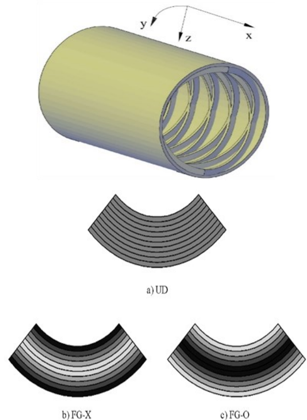
Fig 1. Configuration of the spiral stiffened cylindrical shell and graphene distribution laws of FG-GPLRC
