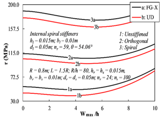
Fig 3. Comparison of dimensionless deflection – torsional load postbuckling curves of unstiffened, orthogonal stiffened and spiral stiffened FG-GPLRC cylindrical shells
