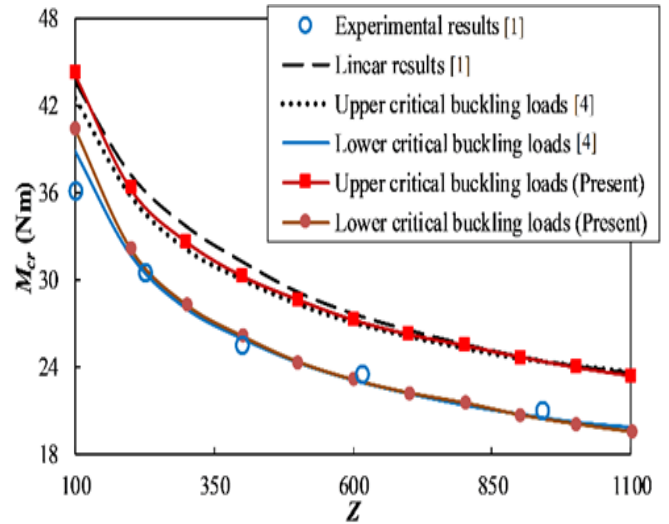
Fig 2. Comparison of critical buckling torsion of isotropic cylindrical shells
