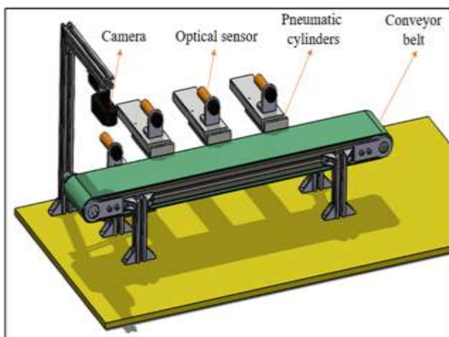
Figure 3. 3D drawing of the sorting system
