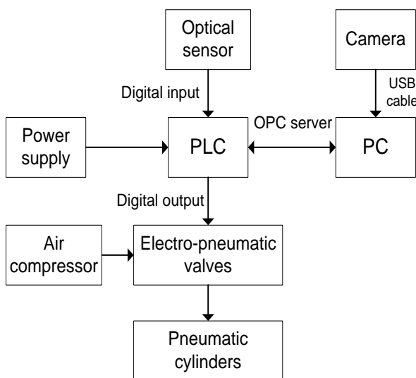
Figure 2. Block diagram of the sorting system
