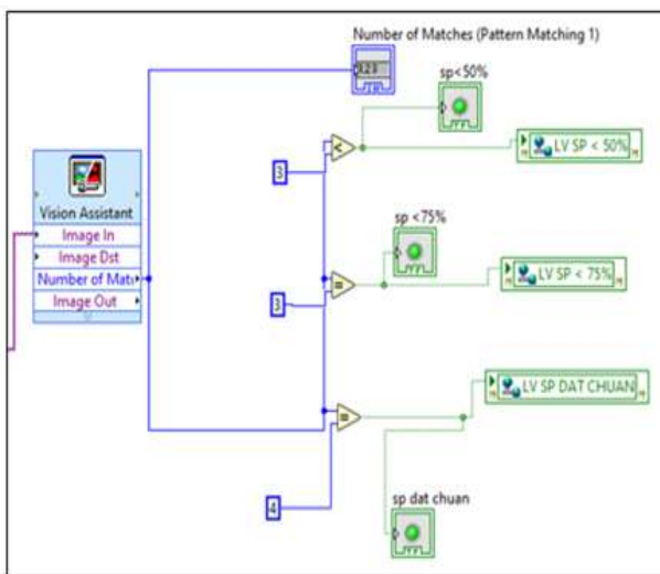
Figure 9. Compare block in LabVIEW
