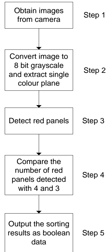
Figure 7. Five steps of image processing
