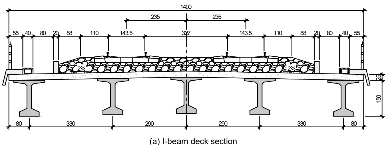
Fig. 1. Typical cross-sectional configurations used in high-speed railway bridges
